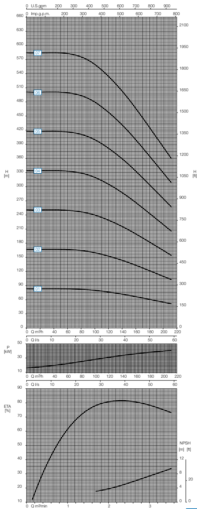
Speed 2950 rpm
