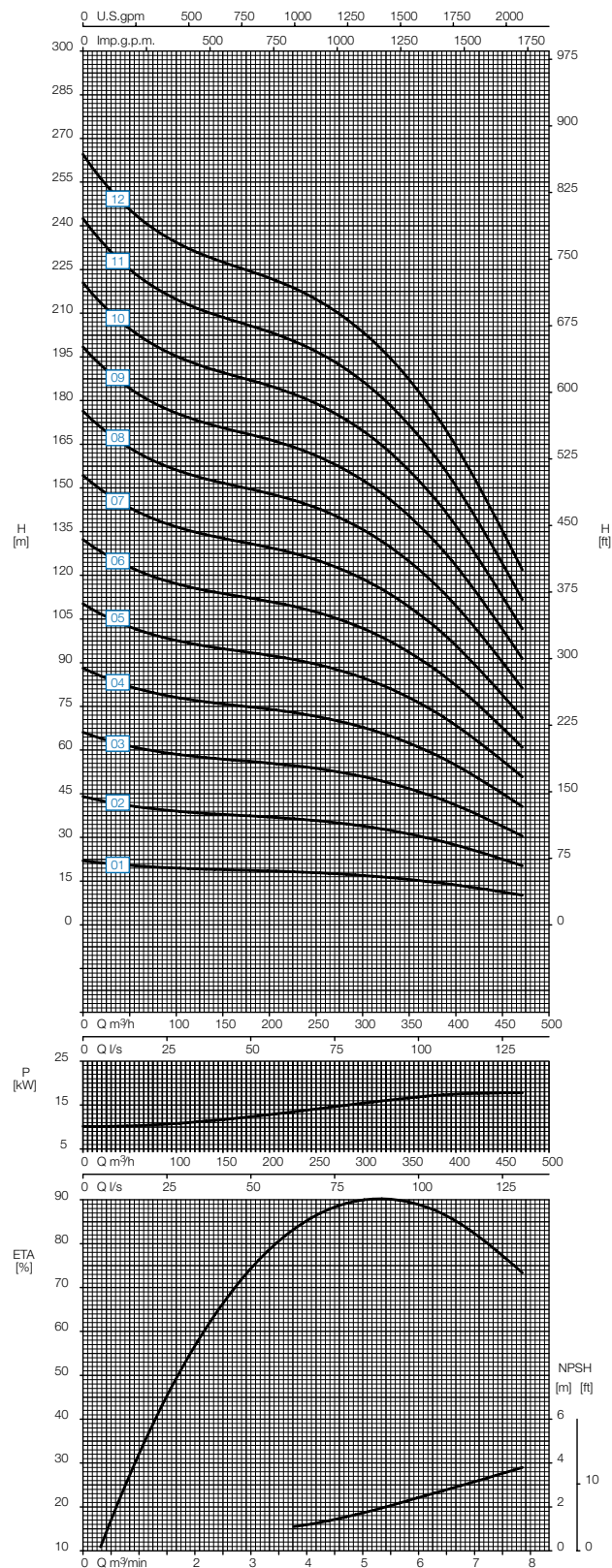
Speed 980 rpm
