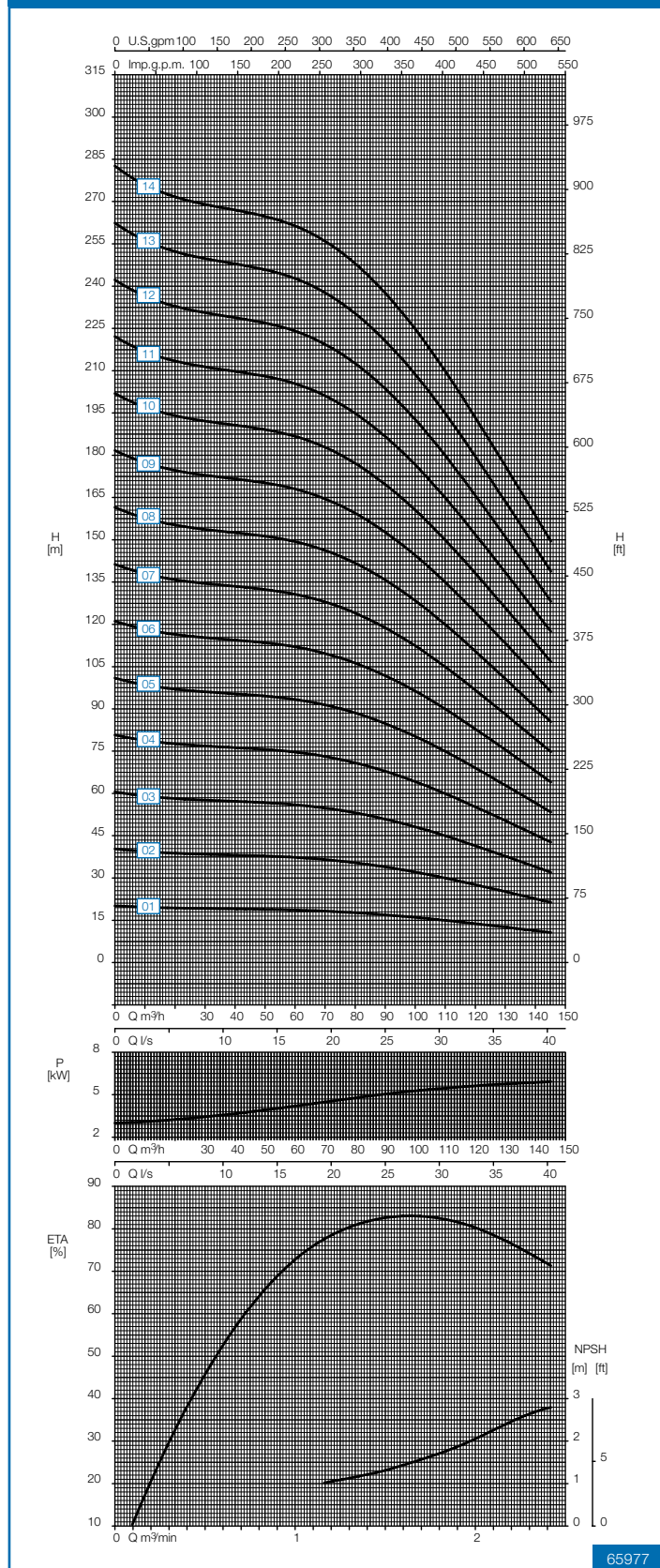
Speed 1450 rpm
