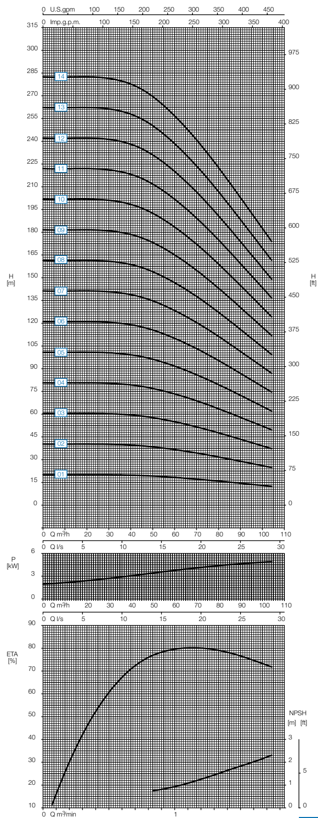
Speed 1450 rpm
