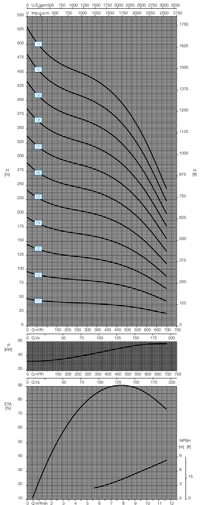
Speed 1450 rpm
