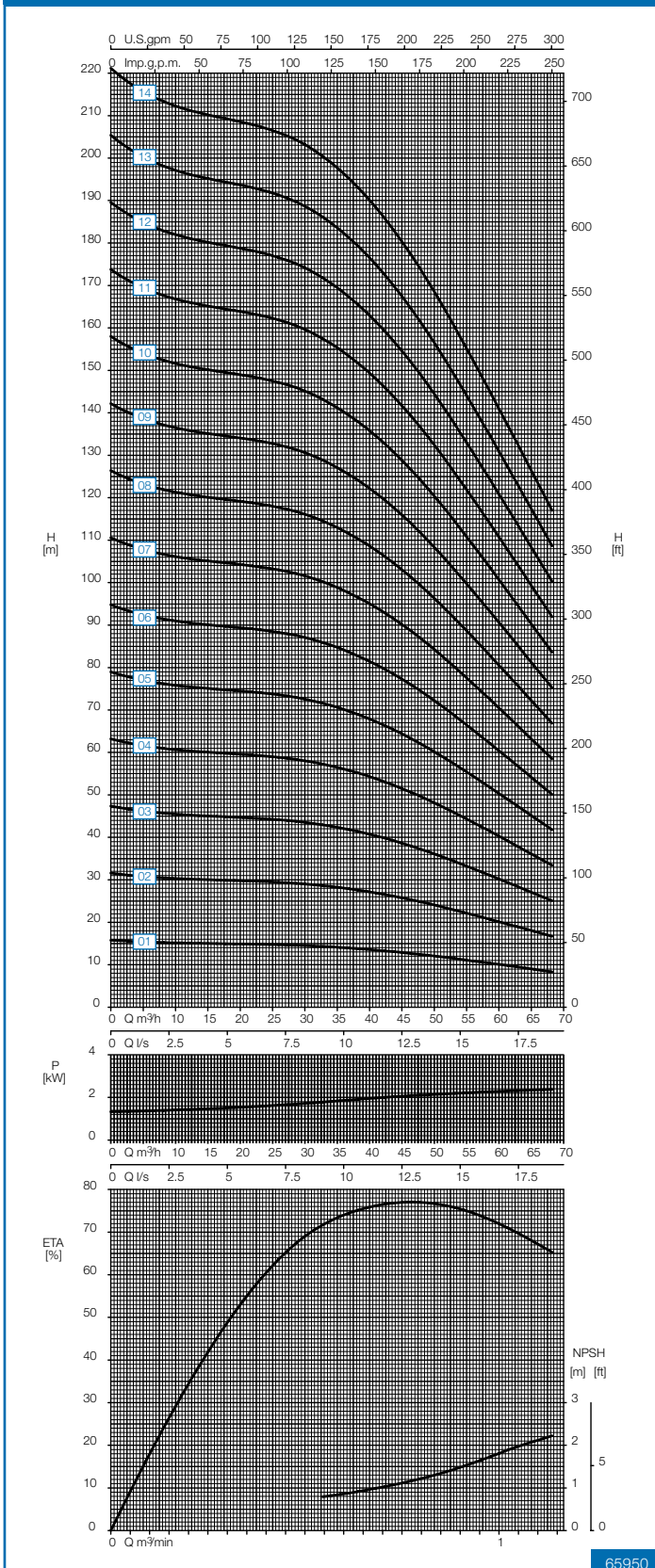
Speed 1760 rpm
