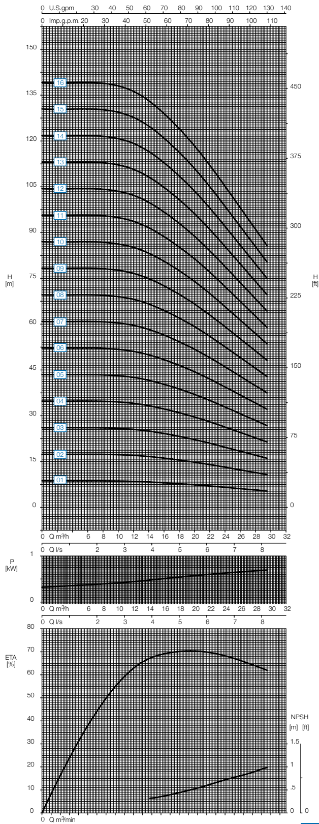
Speed 1450 rpm
