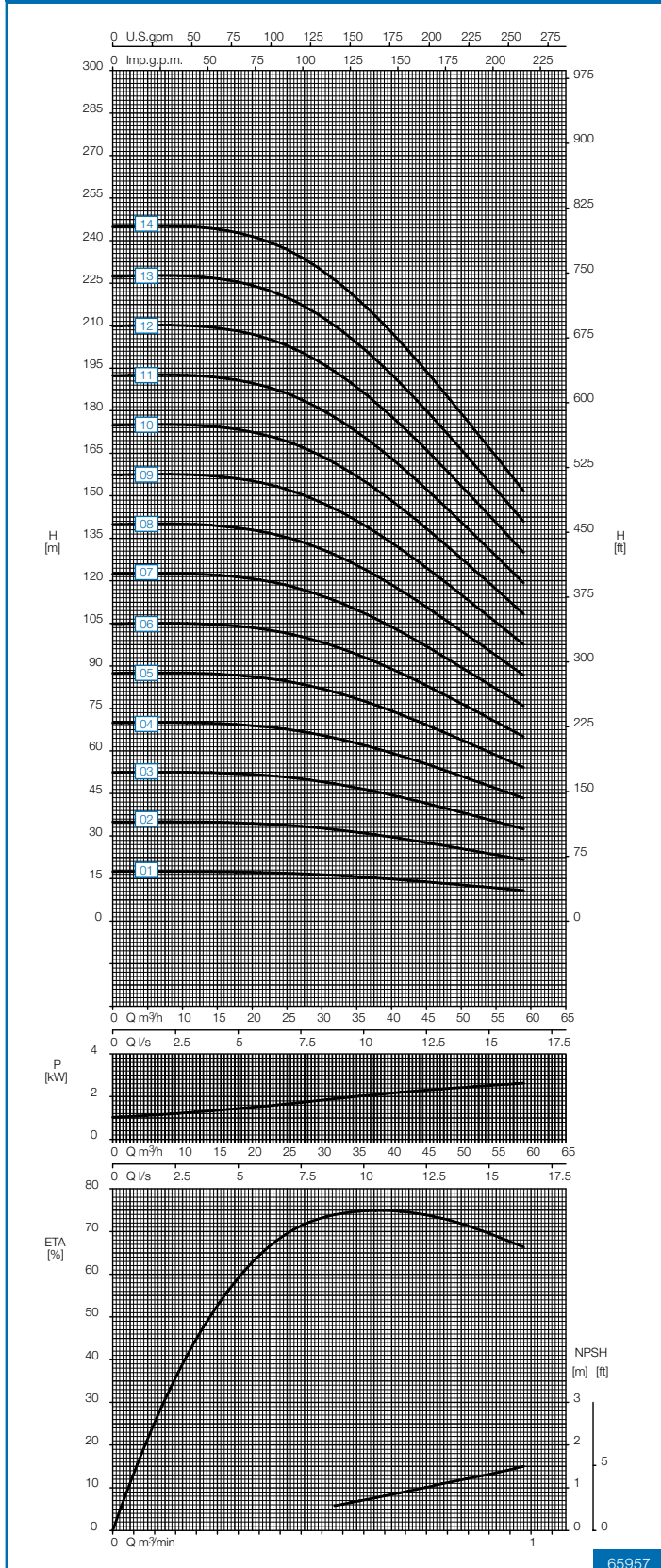
Speed 1450 rpm
