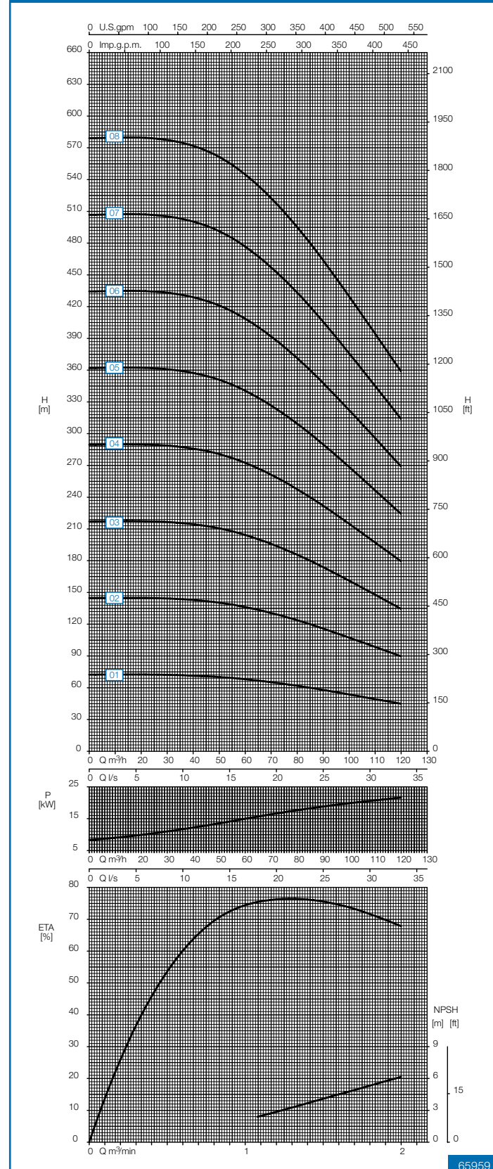
Speed 2950 rpm
