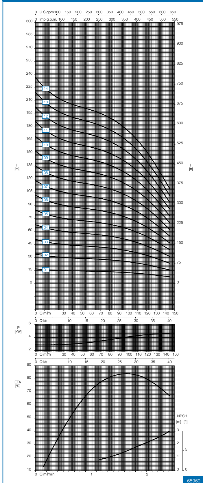
Speed 1450 rpm
