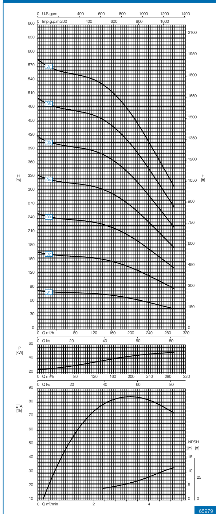
Speed 2950 rpm
