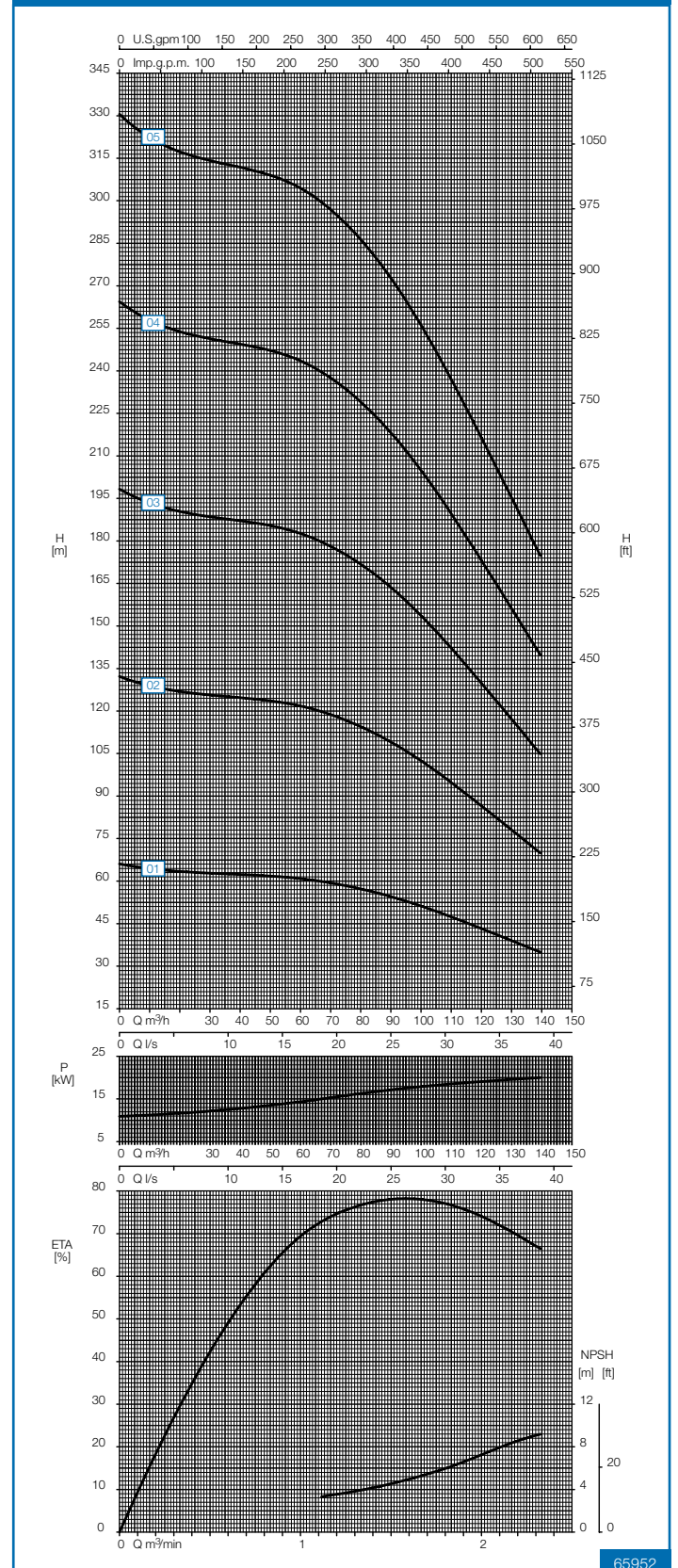
Speed 3600 rpm
