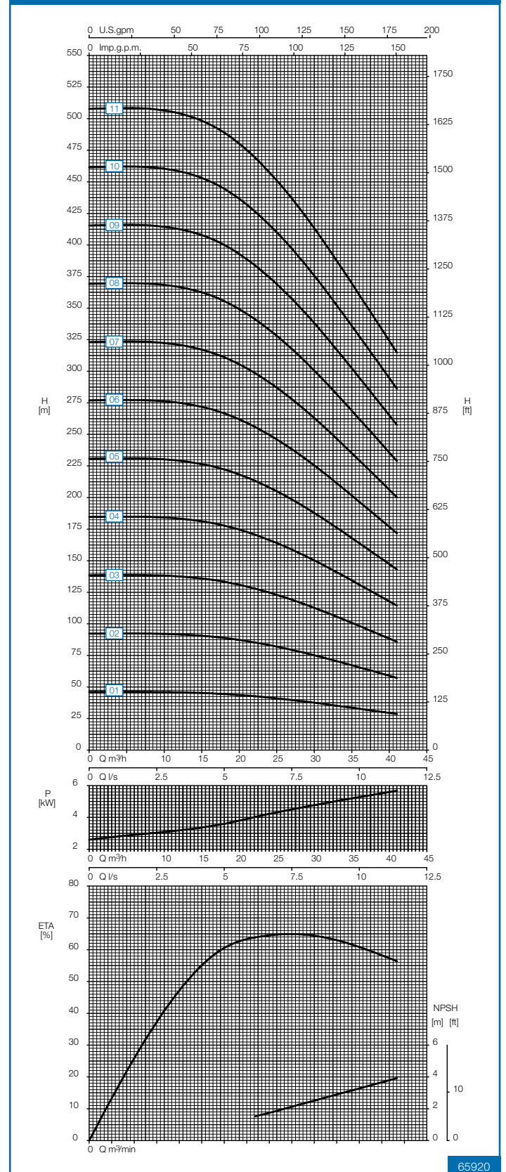
Speed 3600 rpm
