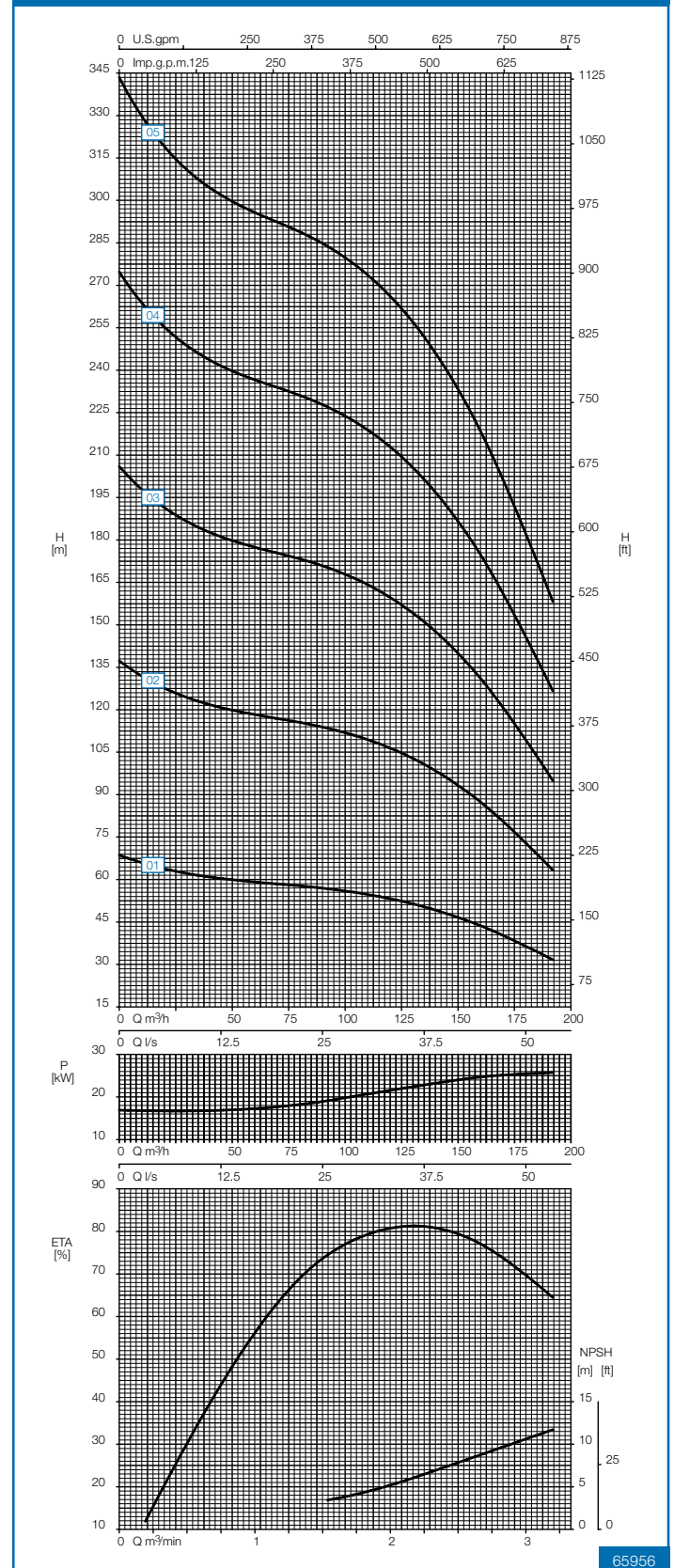
Speed 3600 rpm
