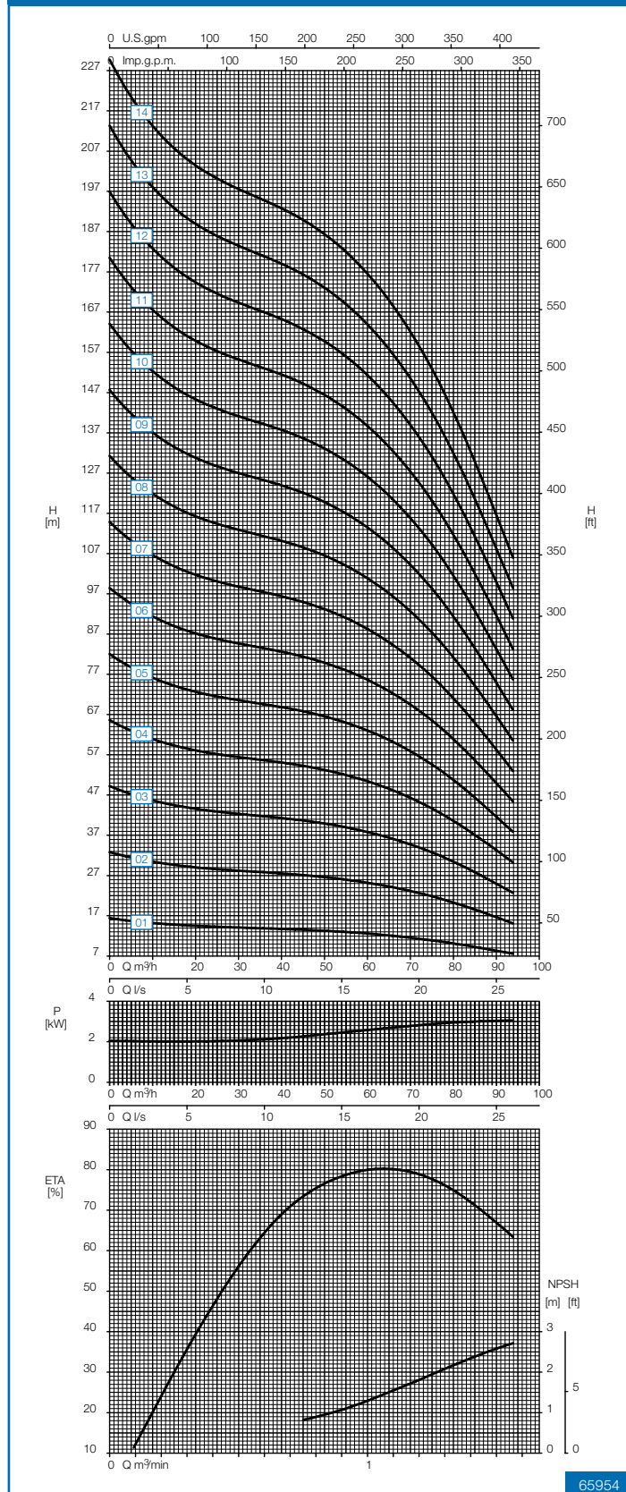
Speed 1760 rpm
