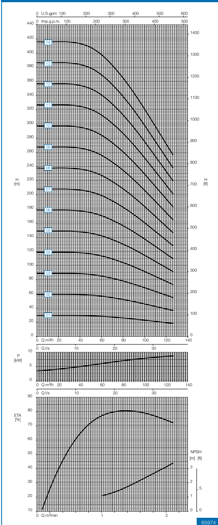
Speed 1760 rpm
