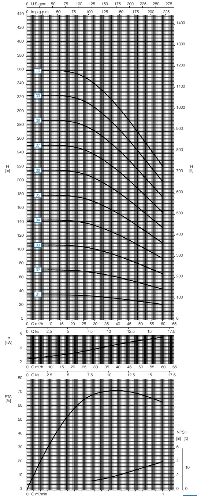
Speed 2950 rpm
